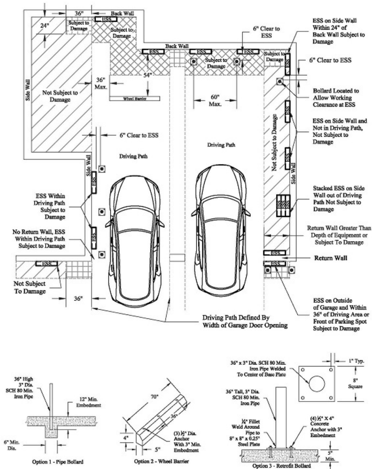
FIGURE 1207.11.7.1 ESS VEHICLE IMPACT PROTECTION
